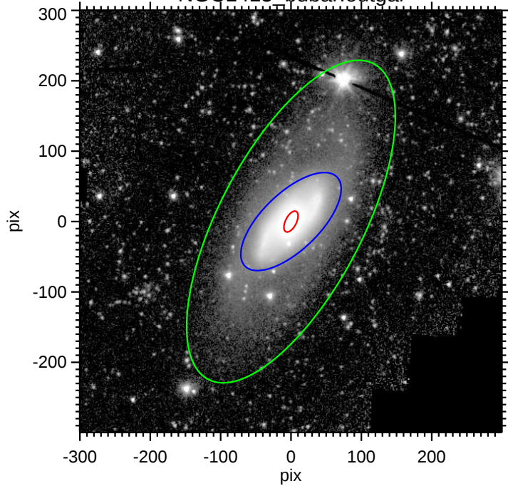
NGC1415_bdbar.outgal
